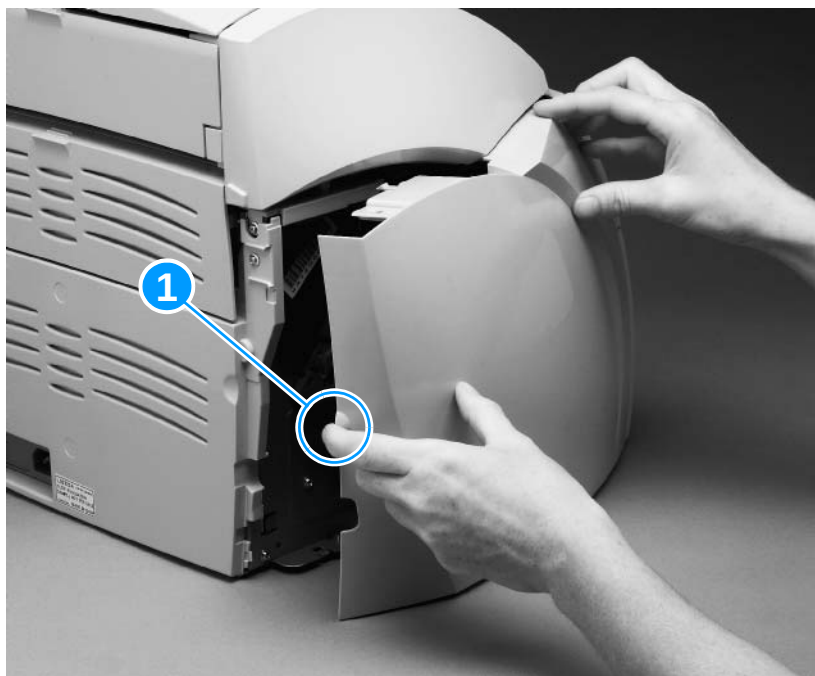
Figure 24. Removing the left side cover
