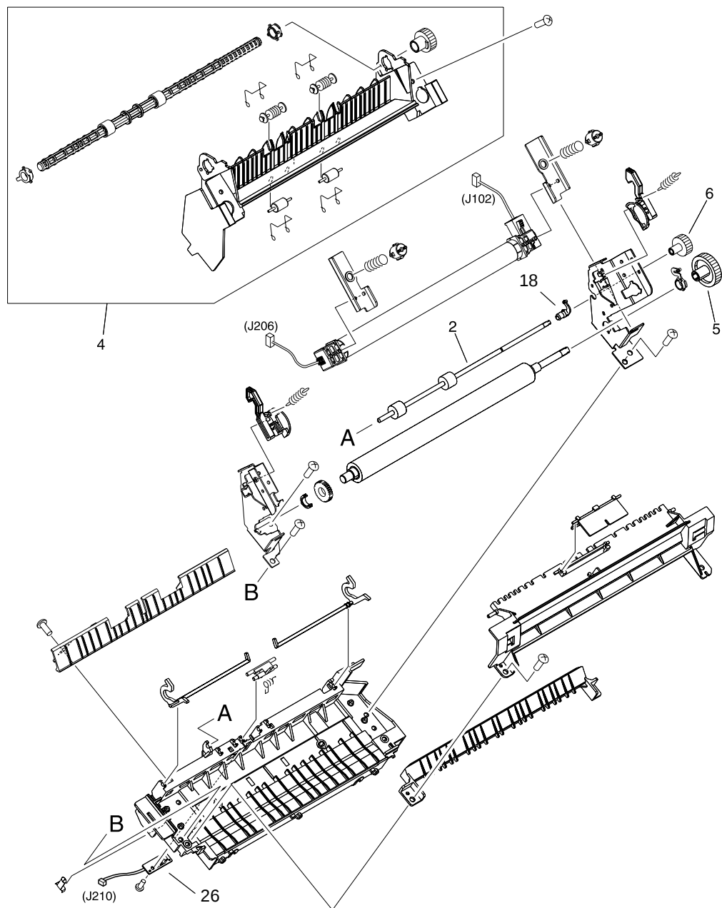
Figure 94. Fuser assembly
